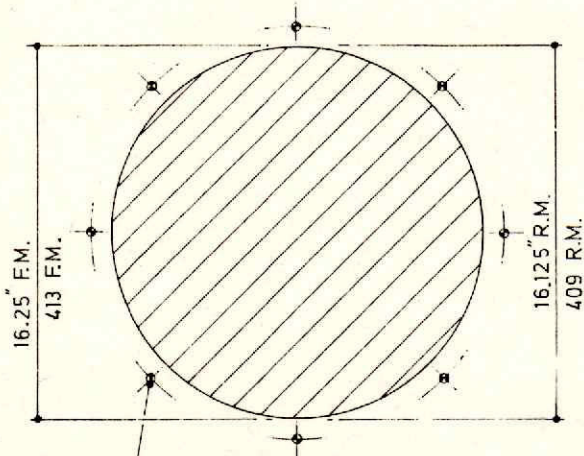
18" CAST ALLOY CHASSIS
