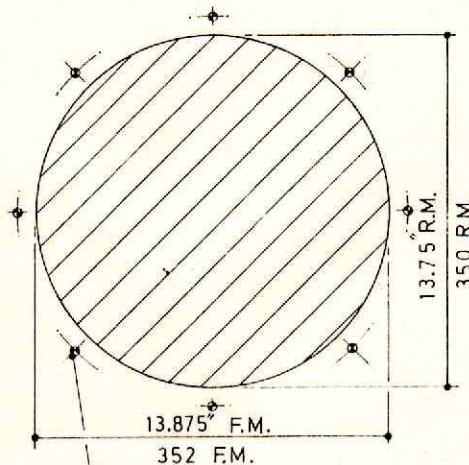
15" PRESSED STEEL CHASSIS
