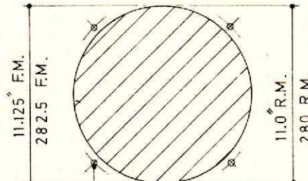
12" PRESSED STEEL CHASSIS
