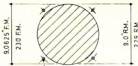
10" PRESSED STEEL CHASSIS
