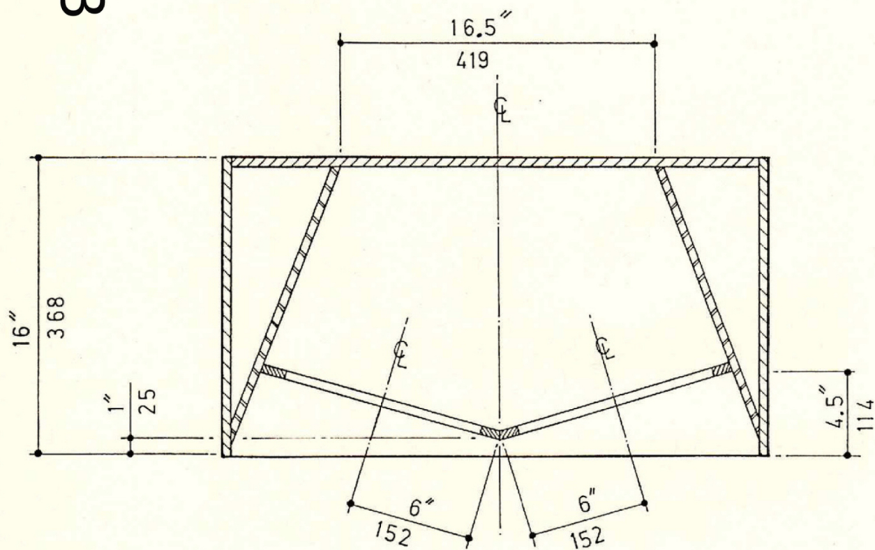
SECTION 'X-X'
